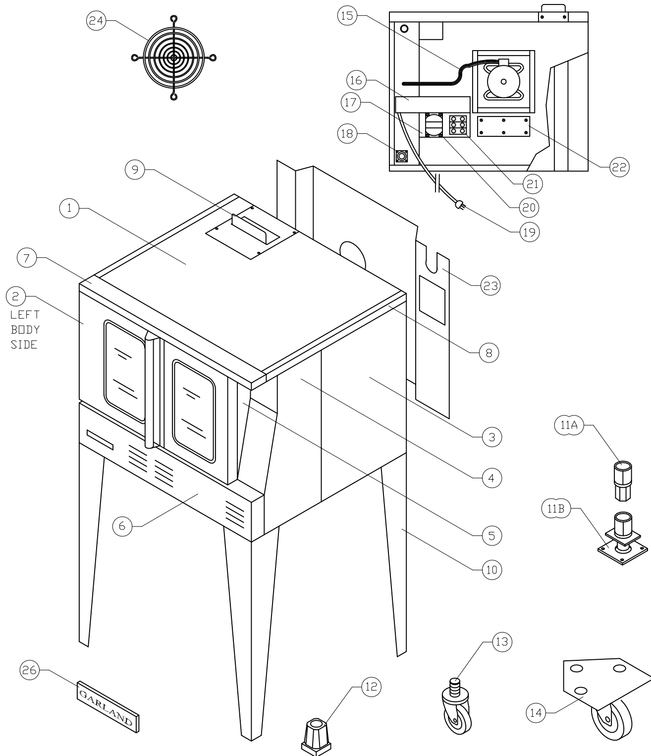
REAR VIEW
