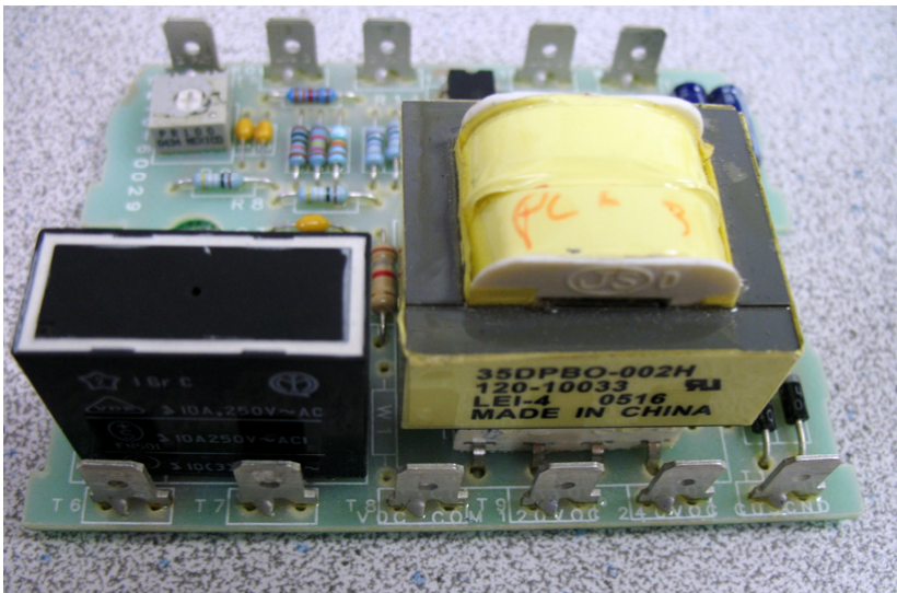
1955501 - Mounted on two standoffs with terminals T1-T11
